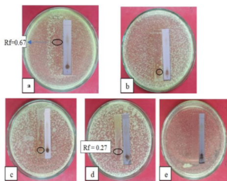
Figure 3 TLC-Bioautography of the extract against (a) E. coli , (b) S. aureus , (c) S. typhi , (d) B. subtilis , and (e) P. aeruginosa
